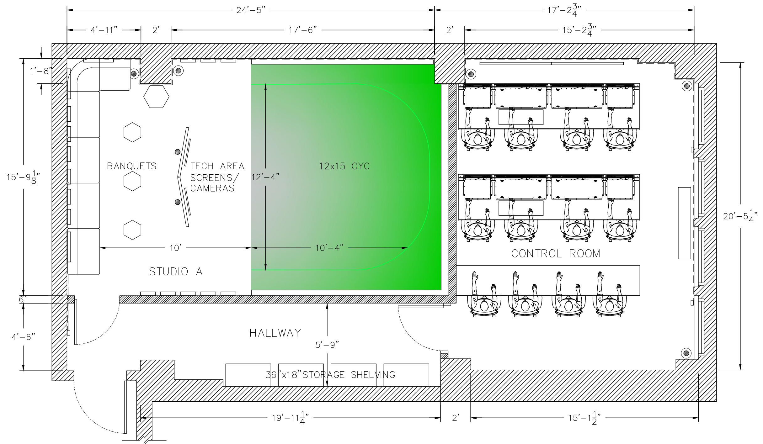
01 STUDIO A & CONTROL ROOM 100 1/4" = 1'-0"
